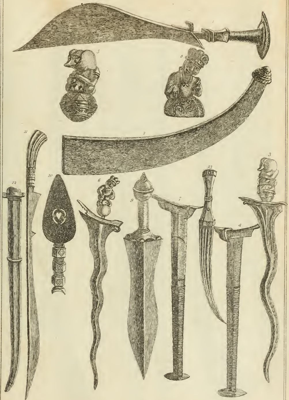
Asiatic Weapons
